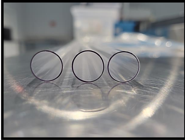
Trimmed on Accu-Trim \text{Ø}.540'' to 42.5'' \pm .125'' Material prone to burrs and cracks
